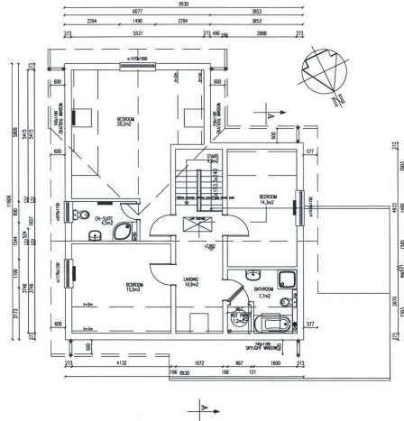
First floor 1:50
