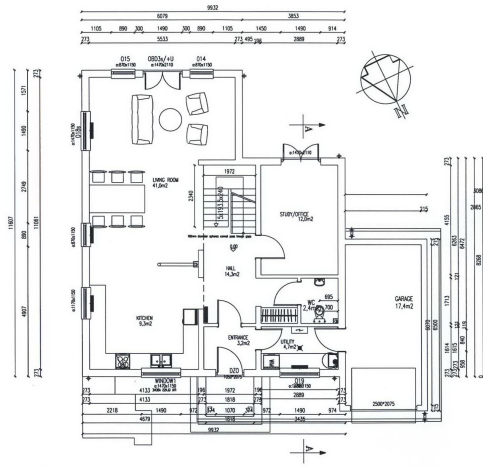
Ground floor 1:50
